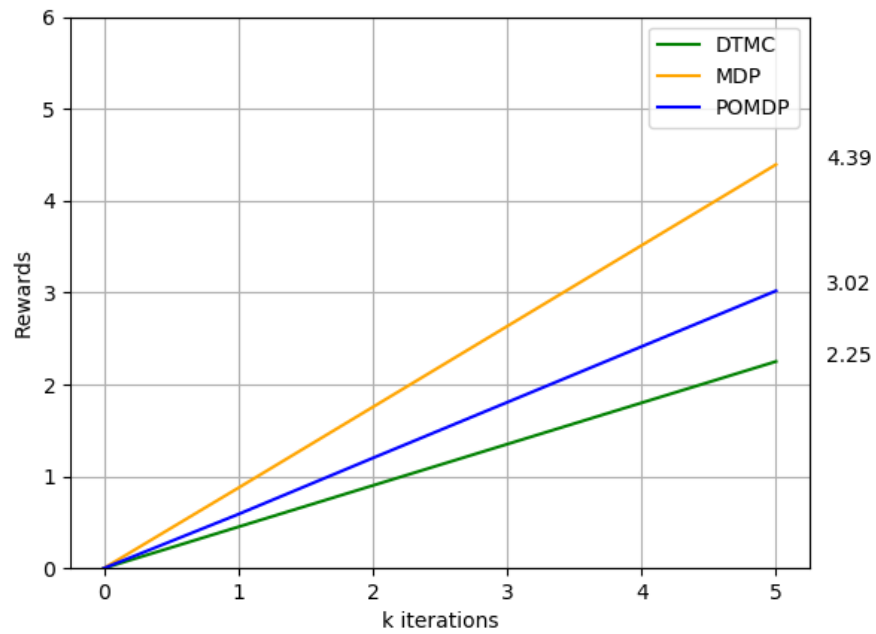
Figure 5.14: Max Rewards of each model (3 bandits) with respect to k iterations
