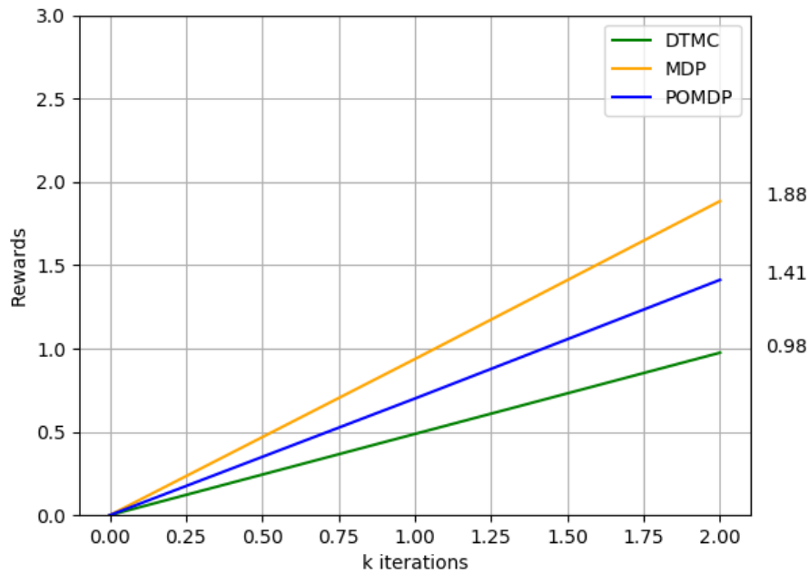
Figure 5.15: Max Rewards of each model (4 bandits) with respect to k iterations
