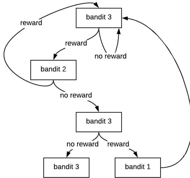
Figure 5.13: Representation of the optimal strategy
