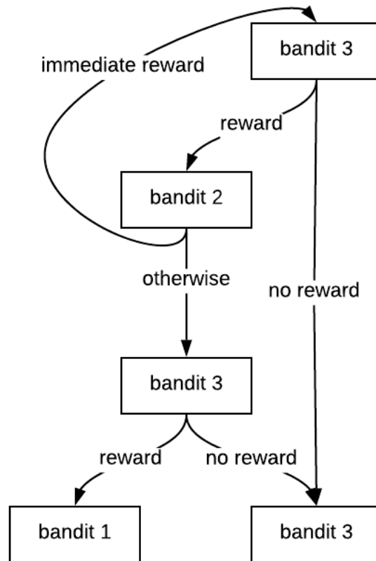
Figure 5.11: Representation of the optimal strategy
