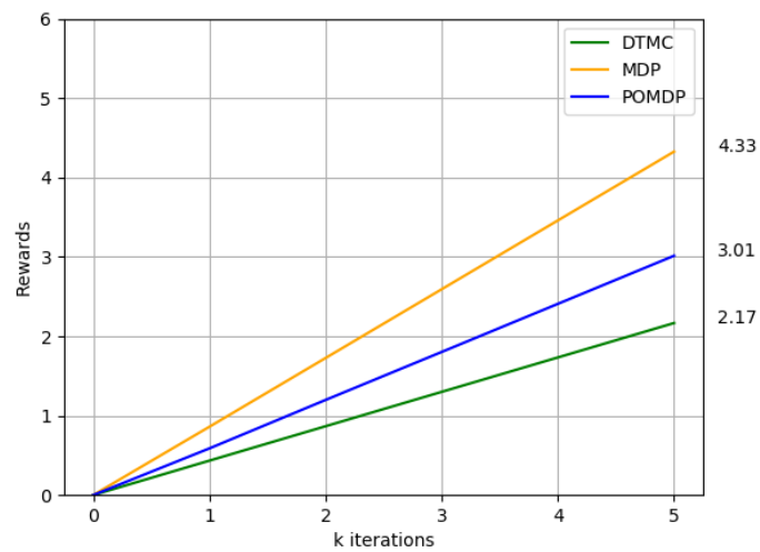
Figure 5.12: Max Rewards of each model (3 bandits) with respect to k iterations
